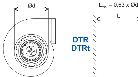
Connection diagrams
